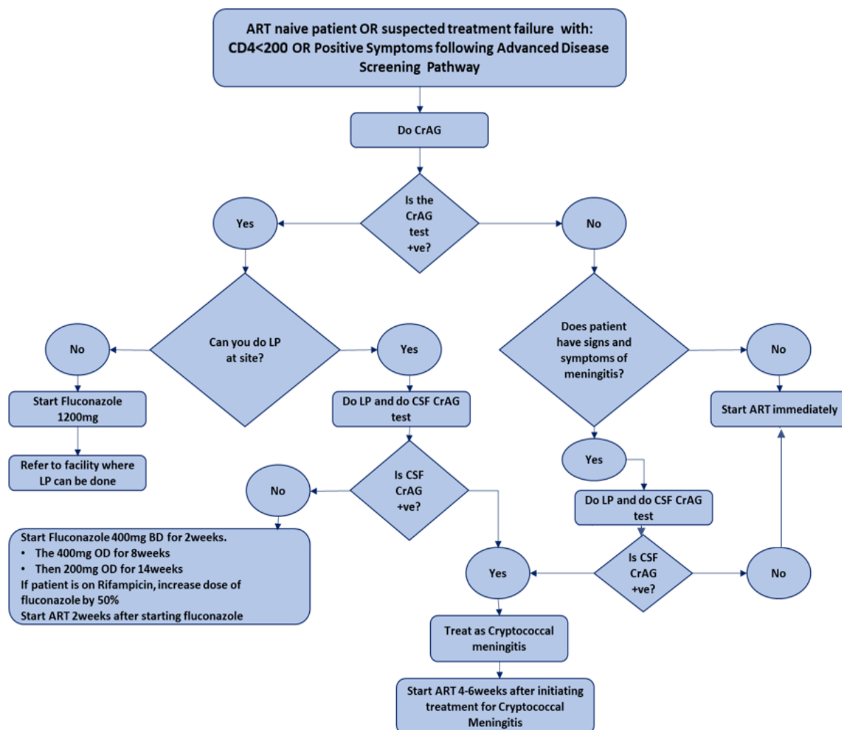
Figure 17: Algorithm for screening and managing Cryptococcal disease
