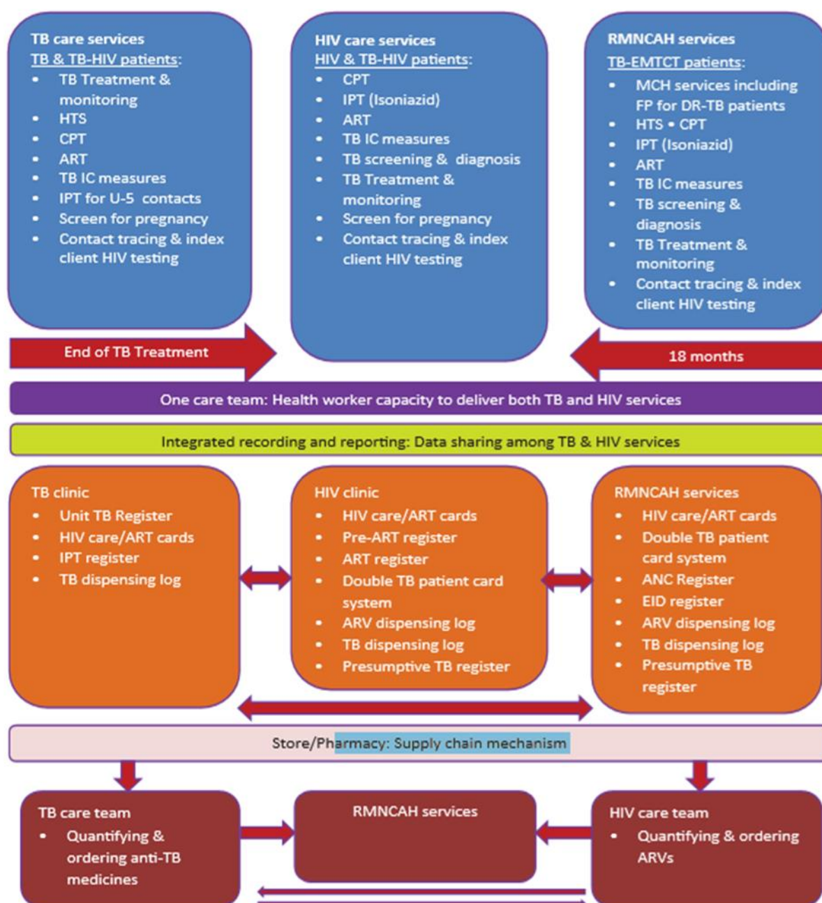
Figure 15: One stop shop model for TBHIV service delivery
